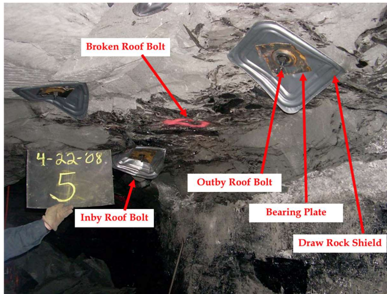
4.2: Roof and rib fall cavity with roof bolts
